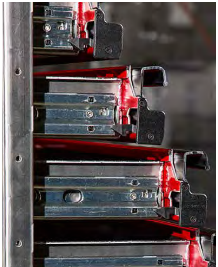
Dual-composite latches, 250 lbs drawer slides
