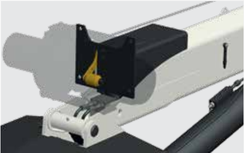
3RD WRAP LIMITER FOR FRICTION LOAD HOLDING Available for PSC 3216 - 6025, 3rd wrap limiters keep 3 wraps of cable around the drum for friction load holding. Exceeds ANSI/ASME requirements.
