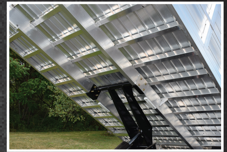
Standard HD Subframe with 12" OC Cross Members
